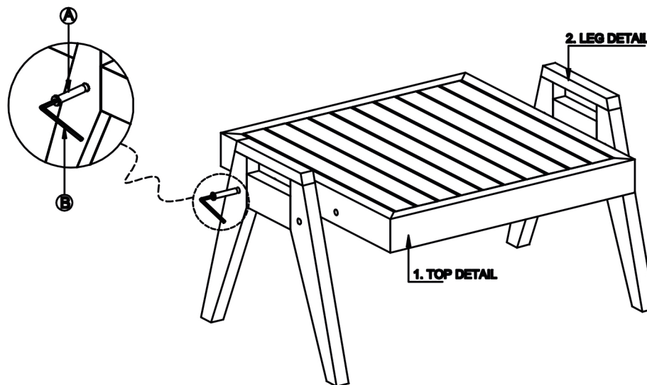
A. Bolt Construction (4 Pcs)
