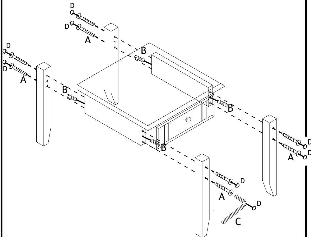
(A) M7 X 50MM X JCBCW SCREW - 8 PCS/SETS
