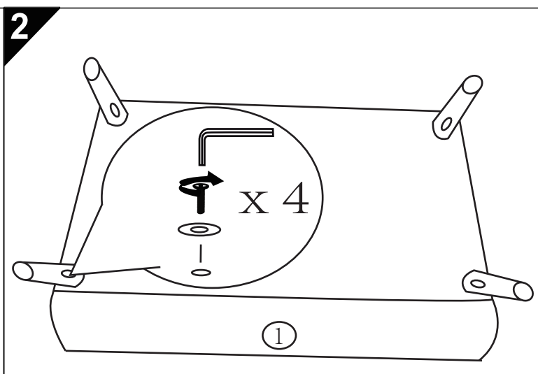
Washer 4x
